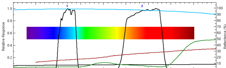
ABI visible spectral bands (black solid lines) and spectral plots for a number of surfaces (snow—light blue; grass—green; dirt—brown; asphalt—black). Higher reflectance is generally "whiter" when enhanced. (Credit: CIMSS and ASTER spectral library)
