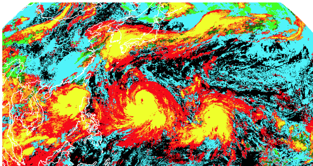
CLEAR LIQUID WATER SUPERCOOLED WATER MIXED PHASE THICK ICE THIN ICE MULTILAYERED ICE CLOUDS
