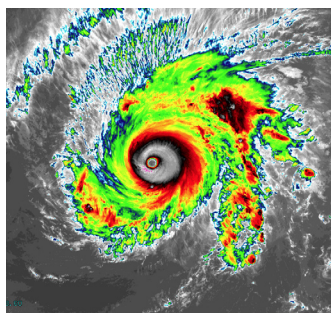
The Advanced Himawari Imager (AHI) 8.6 \mu\text{m} for Typhoon Maysak from March 31, 2015 at 06 UTC. Credit: CIMSS and JMA
