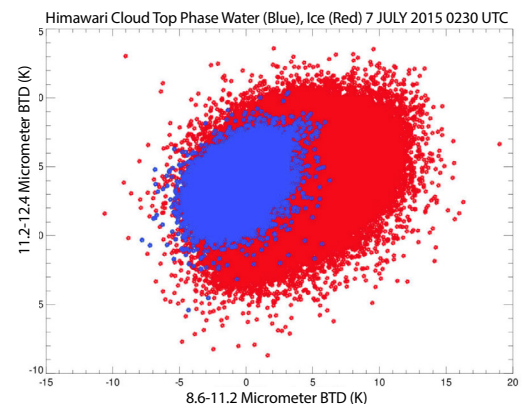
This scatterplot compares brightness temperature differences over an area of both water and ice clouds. Only ice clouds have brightness temperature differences (8.6 \mu\text{m} minus 11.2 \mu\text{m} ) of more than approximately 5 K. Credit: JMA, ASPB, and CIMSS
